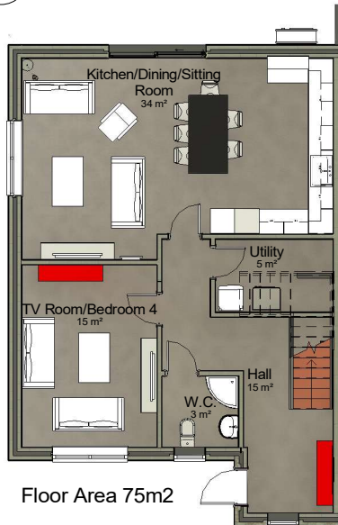
3 Ground Floor Level 1 : 100
